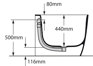
Section BB Shown with K60/61 Waste Kit
