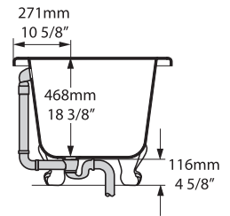
Section BB Shown with K31 Waste Kit
